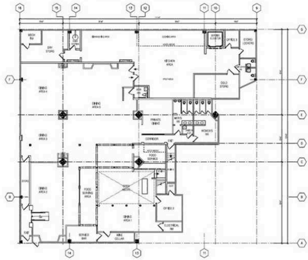
GROUND FLOOR LAYOUT 8,877 SF
